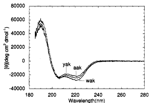
FIGURE 1: Circular dichroism spectra of yak, wak, and aak. Conditions: 0 °C, pH 7, 0.1 M KF, 1 mM potassium phosphate. peptides (Brandts & Kaplan, 1973) and \epsilon_{281\text{nm}} = 5690 \text{ M}^{-1} \text{ cm}^{-1} for tryptophan peptides (Edelhoc, 1967). The NMR method involved collecting one-dimensional ^1\text{H} NMR spectra of standard solutions of a tyrosine peptide (whose concentration had been determined by tyrosine absorbance) and peptide samples of unknown concentration. The standards and samples were dissolved in ^2\text{H}_2\text{O} solutions containing 0.1 mM trimethylsilyl propionate (TMSP). Spectra were collected using a 6000 Hz spectral width. The FID was the sum of 128 scans collected in 16 384 complex data points with a pulse delay of 5 ms. Spectra were processed using FELIX (Hare Research, Inc.) on a Silicon Graphics Personal Iris computer. The areas under the acetylmethyl proton and TMSP peaks of the various ^1\text{H} NMR spectra were integrated, and the areas were expressed as the ratio of the acetyl peak to the TMSP peak. A standard curve of the peak area ratio versus tyrosine peptide concentration was used to determine the concentration of a sample. The standard curve equation was \text{concn (mM)} = 0.288(\text{ratio}) + 0.007 ; R = 0.997 .
